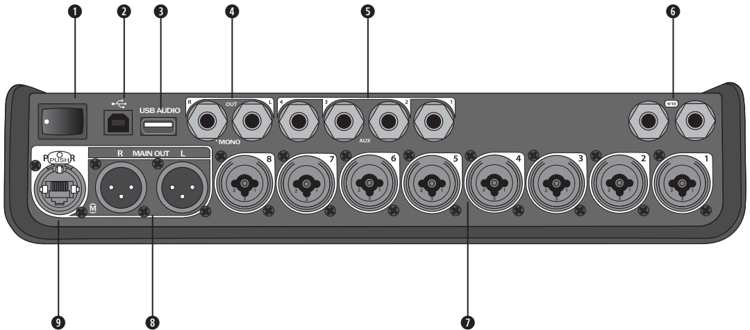
Figure 4. T8S Connection Panel
