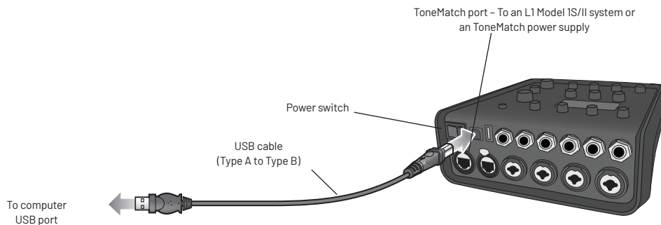
Figure 12. T4S-to-USB connection
